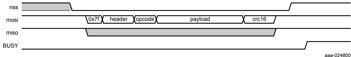
Figure 40. Example SPI WRITE in Secure Firmware Download mode
