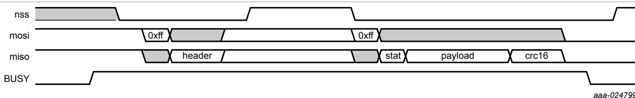
Figure 41. Example SPI READ in Secure Firmware Download mode
