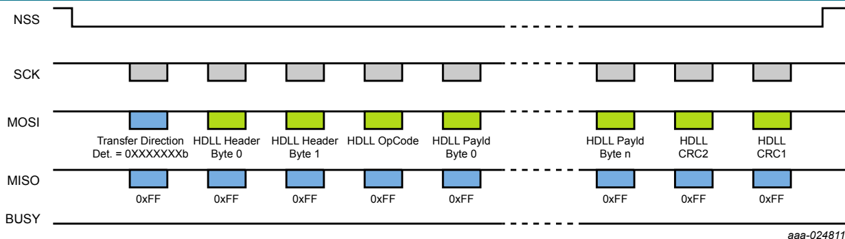
Figure 42. Secure Firmware Download: SPI Write
